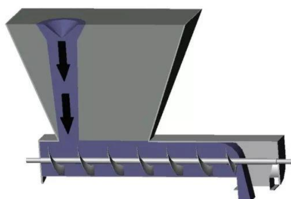
CONSTANT PITCH SCREW FEEDER
